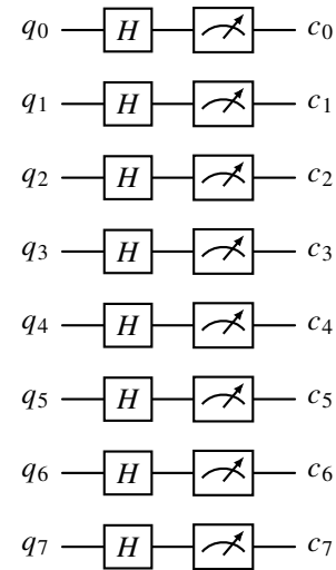
Fig. 2. QRNG circuit: each qubit is placed in superposition via H and immediately measured to produce one random bit.
