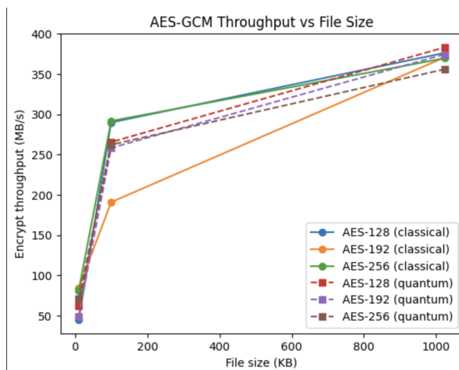
Fig. 6. AES-GCM Encryption On Different Test Cases
