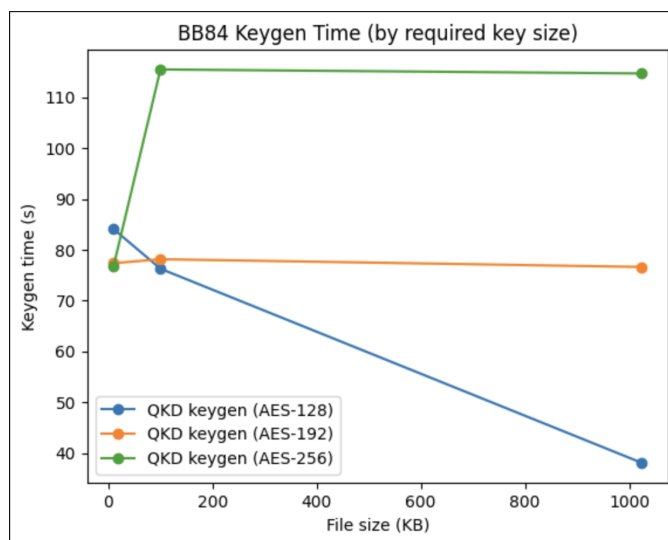
Fig. 7. Time Required for Quantum Key Generation
